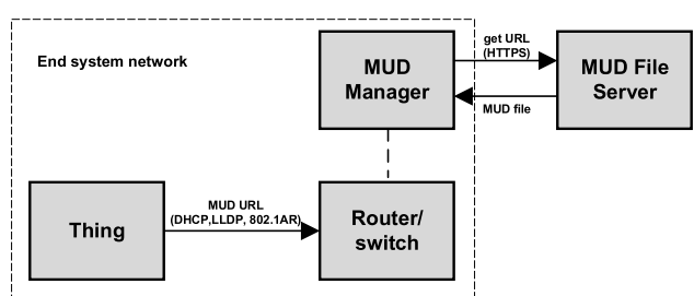
FIGURE 1. MUD architecture [10].
