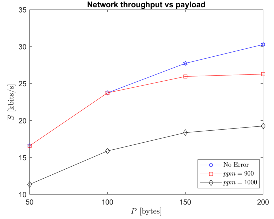
Fig. 6. Network throughput as a function of the payload for different values of ppm characterizing the clocks mounted on tags.
