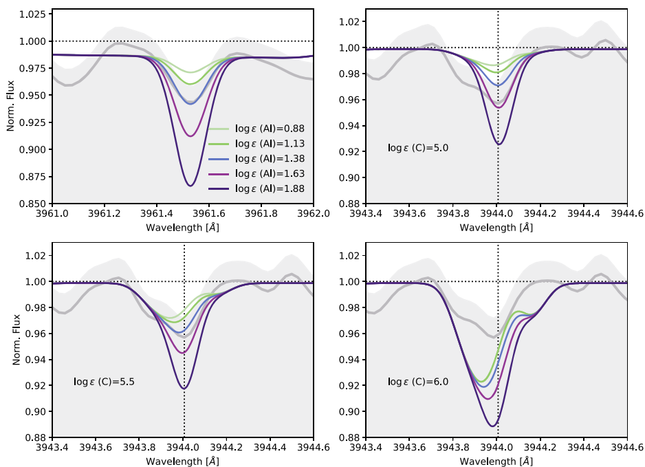
Figure 3. The top left-hand panel shows synthetic spectra with (from the top to bottom) \log \epsilon(\text{Al}) = 0.88, 1.13, 1.38, 1.63, and 1.88 around the Al I line at 3961 Å. The effects of changing aluminium abundances by the same amounts for the modelled spectra around the Al I 3944 Å line are plotted for different carbon abundances \log \epsilon(\text{C}) = 5.0, 5.5, and 6.0 (top right-hand, bottom left-hand, and bottom right-hand panels, respectively). All modelled spectra are smoothed to a resolution of R = 30\,000 . The observed spectrum of Pr 221 is shown as a grey thick line in all panels. The noise level is represented by the grey shaded area.
