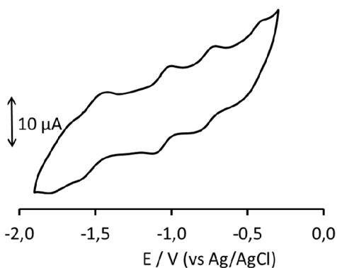
Figure 4. CV profile recorded at the Pt electrode in a \text{CH}_3\text{CN} solution of 1^{6-} . [\text{NBu}_4][\text{PF}_6] ( 0.1 \text{ mol dm}^{-3} ) as the supporting electrolyte. Scan rate of 0.1 \text{ V s}^{-1} .
