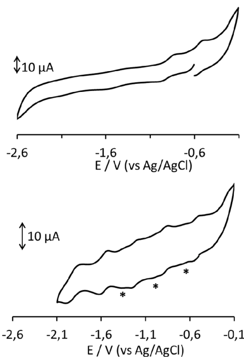
Figure 6. CV profiles recorded at Pt (top) and GC (bottom) electrodes in a \text{CH}_3\text{CN} solution of 3^{5-} . [\text{NBu}_4][\text{PF}_6] ( 0.1 \text{ mol dm}^{-3} ) as the supporting electrolyte. Scan rate of 0.1 \text{ V s}^{-1} . Starred peaks can be attributed to unknown impurities.
