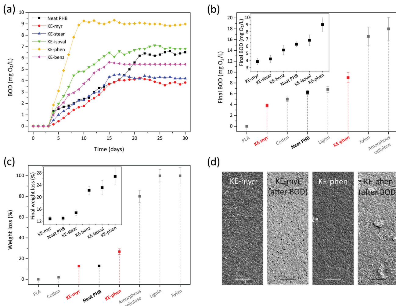
Fig. 6 (a) Typical BOD curves for the KE samples and neat PHB as a function of the immersion time in seawater. (b) BOD 30 values of KE-myristate, KE-phenyl, and neat PHB in comparison to other biopolymers. The inset shows the BOD 30 values of all the KE samples and neat PHB. (c) Weight losses (using eqn (3)) after immersion for 30 days in seawater of KE-myristate, KE-phenyl, and neat PHB in comparison to other biopolymers. The inset shows the weight losses after immersion for 30 days in seawater of all the KE samples and neat PHB. (d) The SEM top-view images of KE-myristate and KE-phenyl samples before and after BOD tests. Scale bar: 25 μm.
