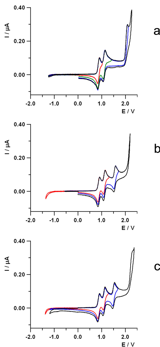
Figure 2. Cyclic voltammetric curves of 0.8 mM porphyrin (a) 1, (b) 2 and (c) 3 recorded in TBAH/ \text{CH}_2\text{Cl}_2 at 298 K; scan rate = 1 \text{V s}^{-1} ; working electrode: platinum disk (diameter 125 \mu\text{m} ); reference electrode: SCE.
