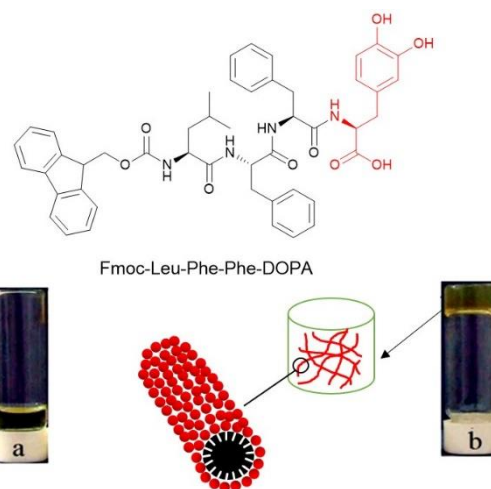
Figure 15. Chemical structures of the (NPC 15199 + Phe-Phe-Dopa) and enzymatic formation of the hydrogelator (Fmoc-Leu-Ohe-Phe-Dopa); a) solution containing 40 mM 1 and 2 with inactive metalloprotease, pH 7.4; b) gel formed with the catalysis of metalloprotease after 5 min.
