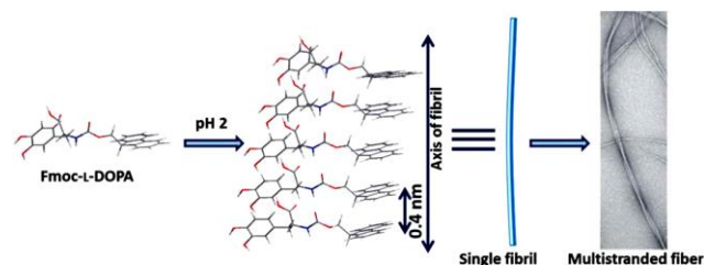
Figure 5. Schematic representation for the proposed model of self-assembly of Fmoc-L-Dopa at pH 2. Adapted with permission from ref. 34. Copyright (2013) Royal Society of Chemistry.
