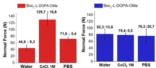
Figure 11. Results for the traction tests of Boc 2 -L-Dopa-OMe and Boc 3 -L-Dopa-OMe
