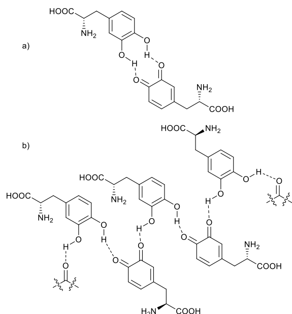
Figure 4. Intermolecular hydrogen bonds between L-Dopa molecules in the reduced and oxidised forms: a) bimolecular hydrogen bonds, b) oligo- or polymolecular hydrogen bonds.
