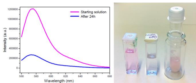
Figure 13. (Left) Emission spectra of an aqueous solution of RhB (2.0 \mu\text{M} ) (pink) and of the same solution after being treated with the ethanol organogel for 24 hours (blue). (Right) Photograph of a fresh sample of the aqueous solution of RhB, of the same sample after treatment with the ethanol organogel, and of the organogel after 24 h (from left to right).
