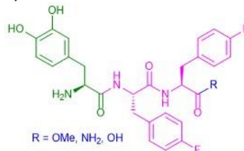
Figure 28. The chemical structure of the peptides of R-COOMe, R-CONH 2 , and R-COOH. Dopa is in green, the antifouling motif, fluorinated phenylalanine, in pink, and the different ending groups, in blue.
