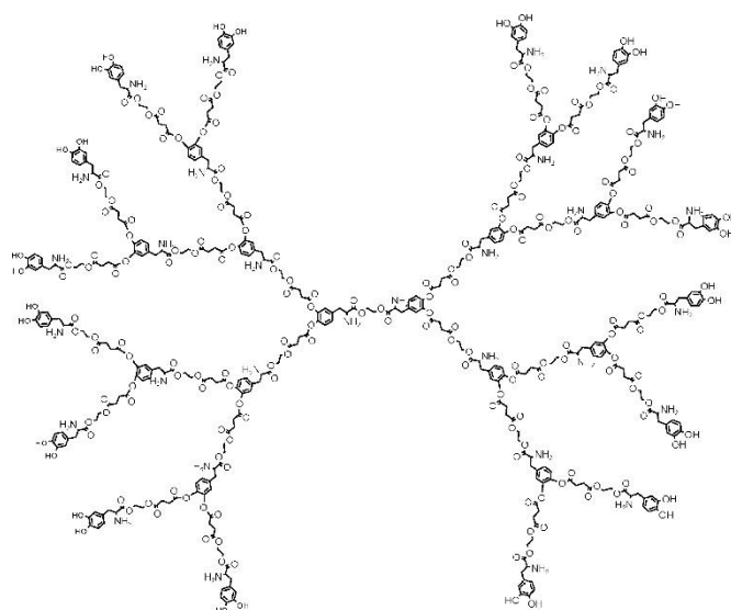
Figure 20. Structure of the second-generation L-DOPA dendrimer produg (HO-G2-NH 2 ). Adapted with permission from ref. 49. Copyright (2006) American Chemical Society.
