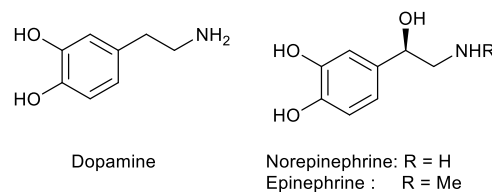
Figure 3. Chemical structure of catecholamines.
