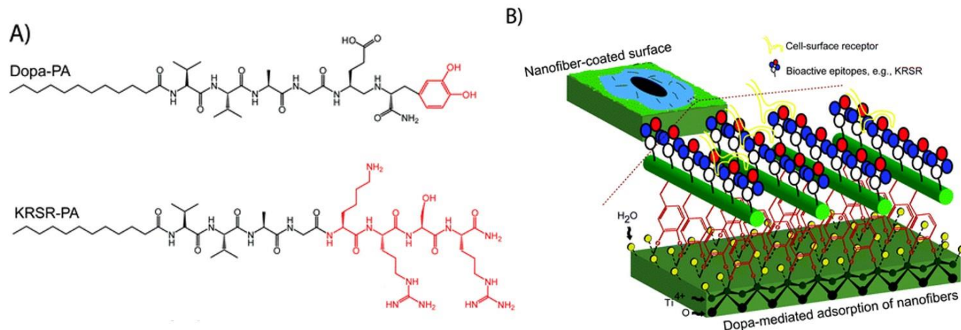
Figure 29. (A) Chemical structures of the peptide amphiphile molecules designed for functionalization of titanium surfaces. (B) Dopa-mediated immobilization of the bioactive nanofibers on titanium surface in the presence of water is shown to occur through catechol–titanium coordination. 58 Adapted with permission from ref. 57. Copyright (2012) Royal Society of Chemistry.
