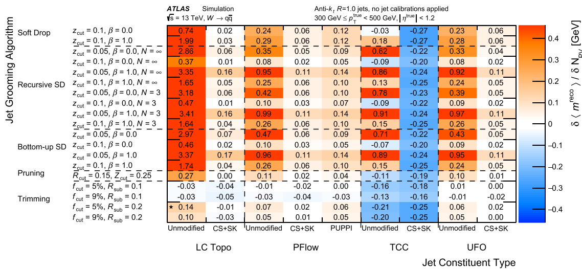
Fig. 12 Pile-up dependence of the value of the fitted W boson mass peak at low p_T . Jet p_T and \eta cuts before tagging are made using the ungroomed particle-level large- R jet matched to each of the groomed reconstructed large- R jets. The current baseline topocluster-based trimmed collection is indicated with a \star . The z -axis colour range is
