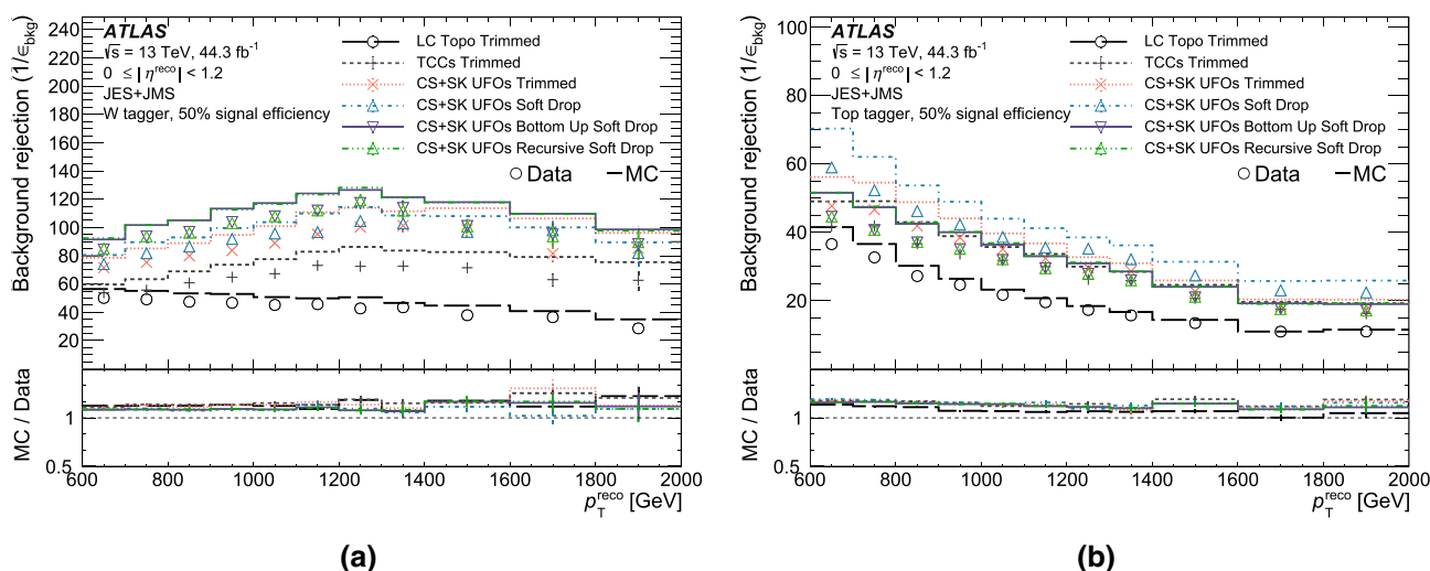
Fig. 21 Data-to-simulation comparisons of the background rejection for groomed jets for a the mass + D_2 W tagger, and b the mass + \tau_{32} top tagger
