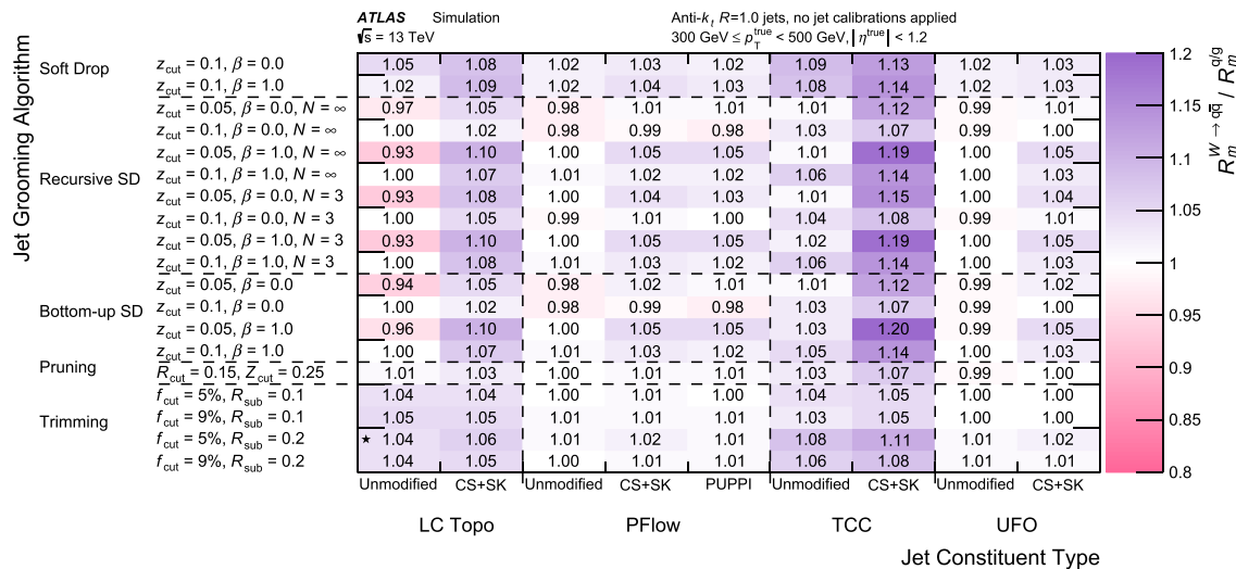
Fig. 14 Ratio of the mean value of mass response in W jets to that in q/g jets at low p_T . Kinematic selections before tagging are made using the ungroomed particle-level large- R jet matched to each of the
