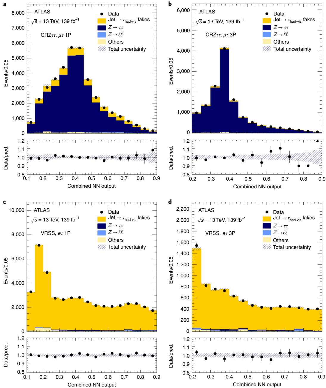
Fig. 1 | Distributions of the combined NN output in control regions and validation regions. a,b, CRZττ for the μτ channel with 1P (a) and 3P (b) τ had-vis candidates. c,d, Same-sign validation region (VRSS) for the eτ channel for events with 1P (c) and 3P (d) τ had-vis candidates. The expected contributions are determined in a fit to data (‘Constraints on \mathcal{B}(Z \rightarrow \ell\tau) ’). The panels below each plot show the ratios of the observed yields to the best-fit background yields. The hatched error bands represent a one standard deviation of the combined statistical and systematic uncertainties. The statistical uncertainties on the data are shown as vertical bars. The last bin in each plot includes overflow events. Similarly good agreement is observed in the same-sign validation region for the μτ channel and CRZττ for the eτ channel, which are not shown here.
