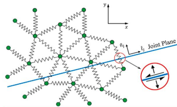
Fig. 1. Schematic representation of lattice array (after [30]).
