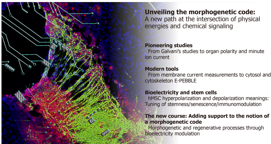
Figure 1 Graphical abstract: Symbolic representation of cellular bioelectronic circuitries in morphogenetic patterning. hMSC: human mesenchymal stem cell.
