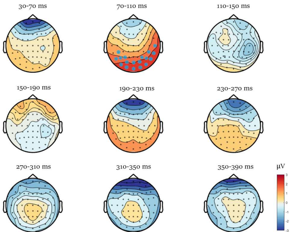
Fig. 3. Results of the cluster-based permutation test comparing the difference (directional – counterphase) ERPs of the long adaptation duration to those of short condition (long difference vs. short difference ). Voltage topographical maps of the grand averaged waveforms (long difference – short difference ) are shown within 40 ms time windows. The electrodes, which were part of the significant spatiotemporal cluster throughout each 40 ms time window, are marked by blue filled circles on the topographical maps. These marked electrodes are O1 , Oz , O2 , PO7 , PO3 , POz , PO4 , PO8 , P7 , P5 , P3 , P4 , P6 , P8 , CP5 , CP6 , TP8 , T8 .
