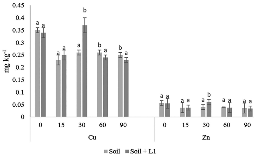
FIGURE 2 Copper (Cu) and Zinc (Zn) concentrations (mg kg -1 ) in the soil after 0, 15, 30, 60 and 90 days of incubation with or not L1 yeast strain suspension (10 8 cells ml -1 ) at room temperature. Each value is the mean of three replicates. Same letters within the comparison of the different treatments at the same time are not statistically significant according to the LSD test ( p < .05 )
