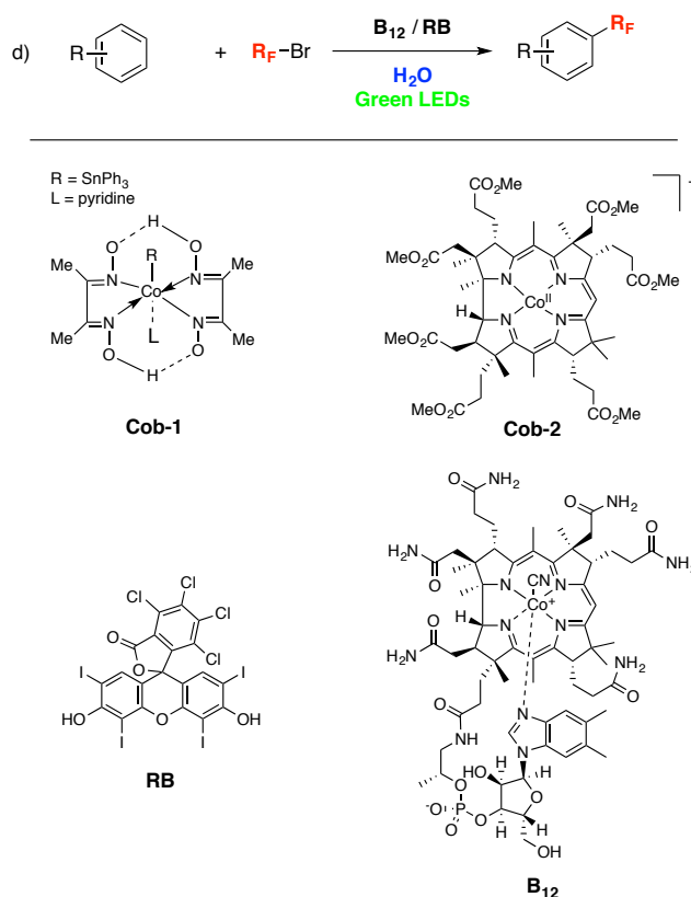
Scheme 2. Co-catalysed fluoralkylation reactions
