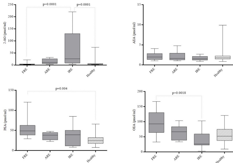
FIGURE 2 | Plasmatic concentrations of 2-arachidonoylglycerol (2-AG), N-arachidonylethanolamine (AEA), N-palmitoylethanolamine (PEA) and N-oleoylethanolamine (OEA) in healthy dogs and in dogs affected by Food-responsive Enteropathy (FRE, n = 10 ), Antibiotic-responsive Enteropathy (ARE, n = 9 ) and Immunosuppressive-responsive enteropathy (IRE, n = 14 ). Boxes show interquartile ranges with median values represented by the central lines, and minimum and maximum values represented by the endpoints of vertical lines.
