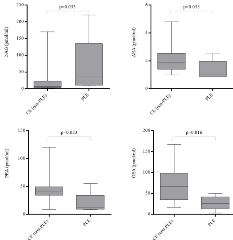
FIGURE 3 | Plasmatic concentrations of 2-arachidonoylglycerol (2-AG), N-arachidonylethanolamine (AEA), N-palmitoylethanolamine (PEA) and N-oleoylethanolamine (OEA) in dogs affected by chronic enteropathy with ( n = 5 ) and without ( n = 28 ) loss of proteins across the gut. CE, Chronic Enteropathy; PLE, Protein-Losing Enteropathy. Boxes show interquartile ranges with median values represented by the central lines, and minimum and maximum values represented by the endpoints of vertical lines.
