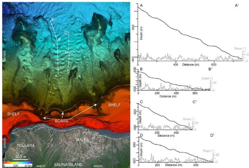
Figure 7 Shaded relief map of the Northern Salina channel, where the bedforms field Sal1 (location in Fig. 1 and 1 ESM) is recognizable; on the right, bathymetric sections (dark line) and slope gradients (grey-line) extracted from the DEM are showed
