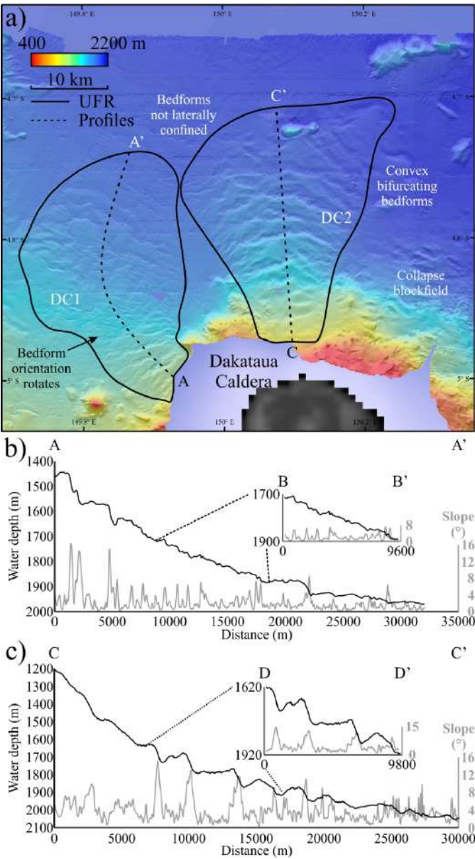
Figure 4. a) Map of bedforms surrounding Dakataua Caldera. Bedform fields included in Table 1 are indicated. UFR = Upper-Flow Regime. b – c) Bathymetric profiles and slope gradients along the profiles of the bedform fields identified in a).
