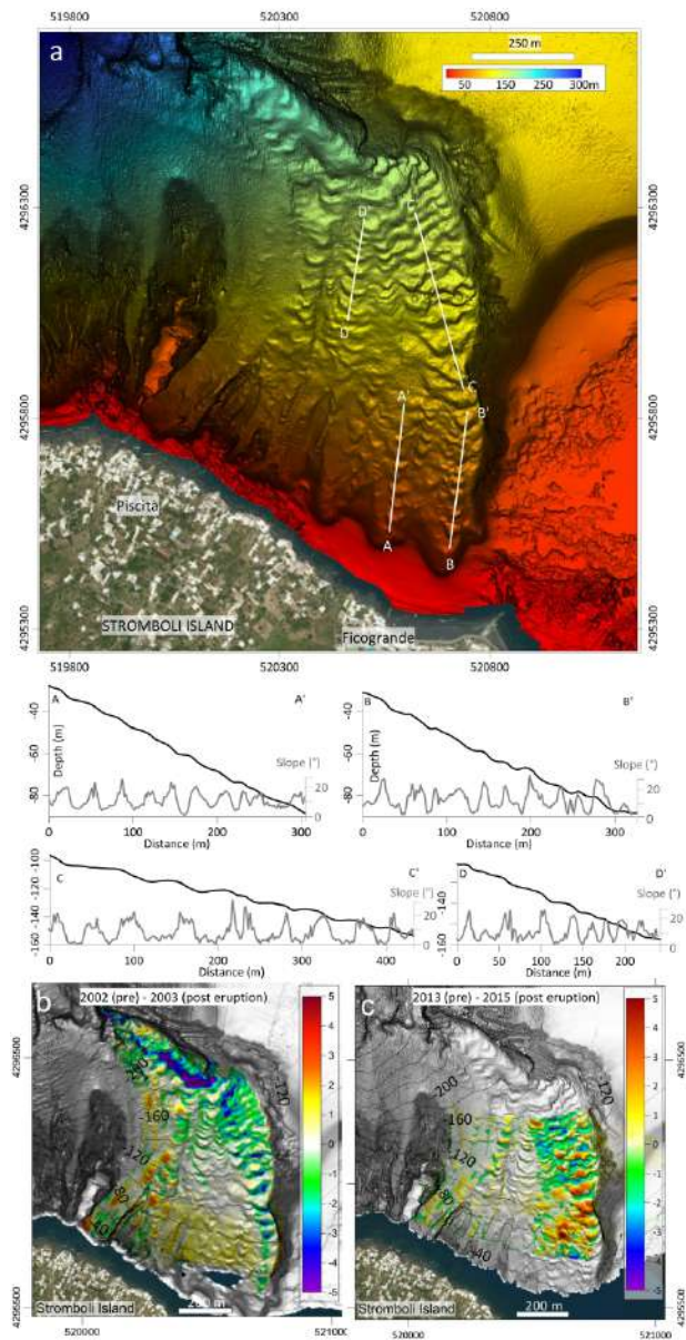
Figure 6 a) Shaded relief map of the Piscit  channel, where the bedforms field Str4 (location in Fig. 1 and 1ESM) is recognizable; below, bathymetric sections (dark line) and slope gradients (grey-line) extracted from 2013 DEM are showed. b) Residual map between 2002 and 2003 bathymetries collected before and after the Stromboli 2002 eruption and tsunamigenic landslide, evidencing a main migration of bedforms on the eastern side of the channel. c) Residual map between 2013 and 2015 bathymetries collected before and after the 2014 Stromboli eruption, showing the migration of the bedforms mainly on the eastern side of the channel.
