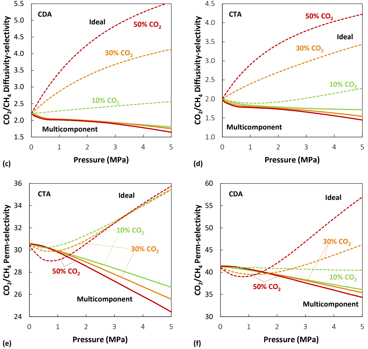
Figure 13. \text{CO}_2/\text{CH}_4 solubility-selectivity, diffusivity-selectivity and perm-selectivity in CDA and CTA calculated with the NELF and ST models at 35 °C and at different mixture compositions: 10/90 mol% in green, 30/70 mol% in orange, 50/50 mol% in red. Dashed lines represent the ideal solubility-selectivity calculated with pure gas data.
