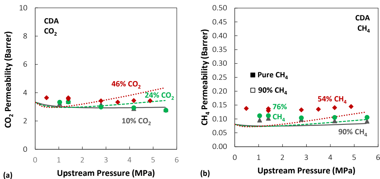
Figure 9. Permeability of \text{CO}_2 (a) and \text{CH}_4 (b) in CDA at 35 °C. Experimental data from ref. [82] are shown: red diamonds 46% \text{CO}_2 -54% \text{CH}_4 mixture, green circles 24% \text{CO}_2 -76% \text{CH}_4 mixture, gray triangles 10% \text{CO}_2 -90% \text{CH}_4 mixture. Mixed gas data for \text{CH}_4 pure and mixed gas permeation from [61] are shown with squares in (b) for comparison, to exemplify the variability in \text{CH}_4 permeability. Lines represent ST model predictions: solid 10% \text{CO}_2 , dash 24% \text{CO}_2 , dot 46% \text{CO}_2 .
