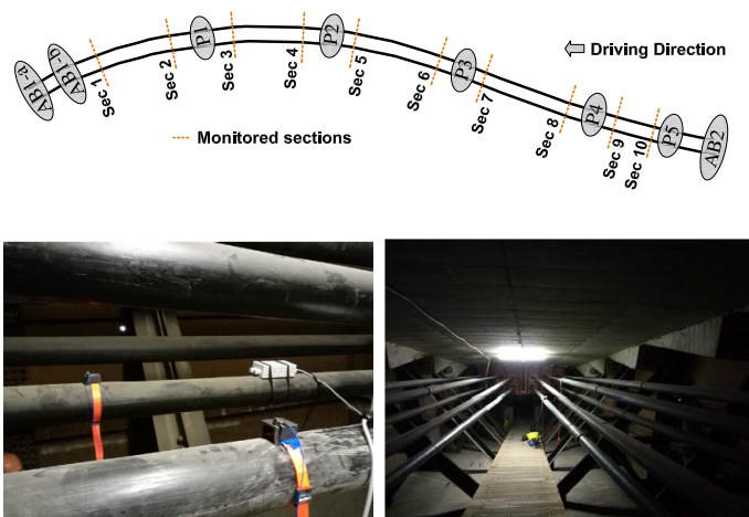
Fig. 1. Monitoring system installation: (1) Plan view of the monitored highway viaduct. (2) MEMS accelerometers installed on the external steel tendons. (3) External prestressing tendons.
