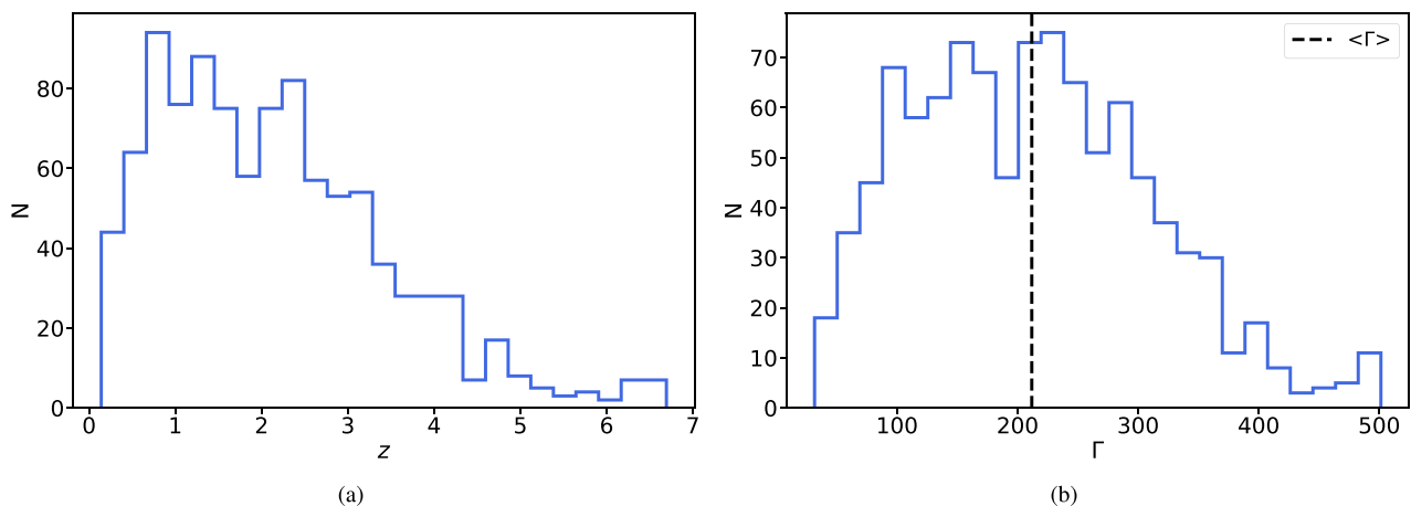
Figure A2. (a) Distributions of the redshift z values randomly extracted for GRB08102853. (b) Corresponding bulk Lorentz factor \Gamma values obtained by using the correlation in equation (2) (Lü et al. 2012). The black dashed line shows the average \Gamma of the considered GRB, \langle \Gamma \rangle \simeq 210 .
