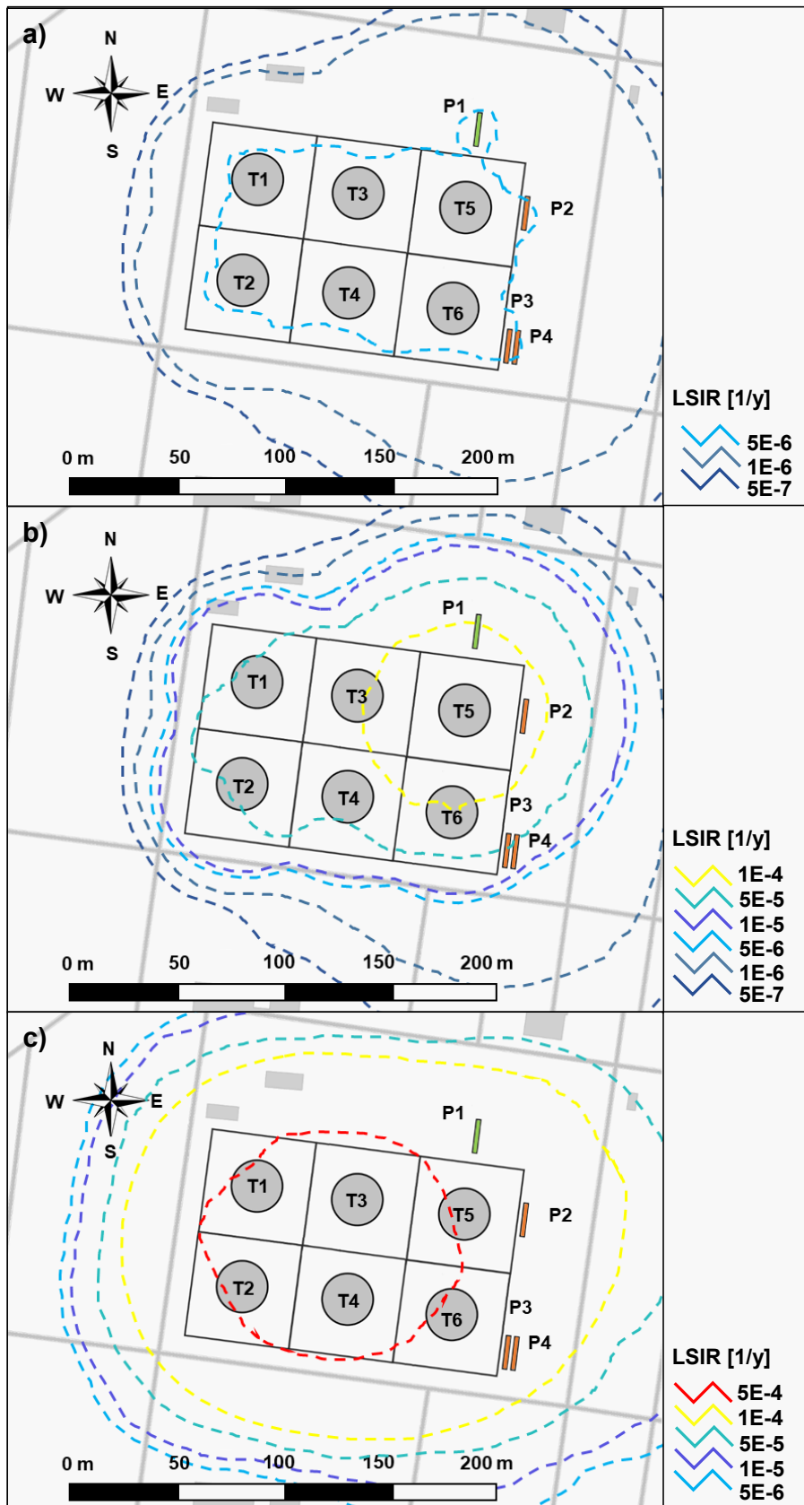
Figure 5: a) Local-Specific Individual Risk (LSIR) contours obtained considering only conventional scenarios; b) LSIR contours obtained considering conventional and primary lightning-induced Natech; c) LSIR contours obtained considering conventional scenarios, primary Natech scenarios and overall escalation scenarios.
