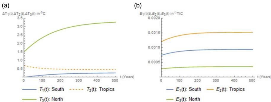
Figure 2. Paths for optimal temperature anomalies (left panel) and emissions (right panel) for scenario S4, Rb1.
