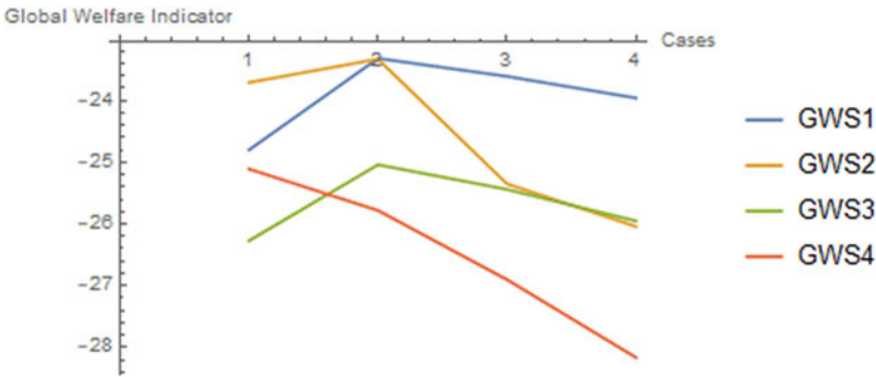
Figure 3. Evolution of global welfare indicators (GW) for S1, . . . , S4 when preferences for robustness increase. Note: On the horizontal axis, 1 is D, 2 is Rb1, 3 is Rb2 and 4 is Rb3.
