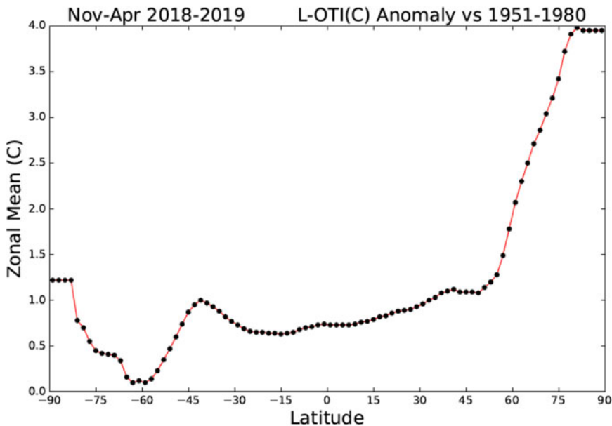
Figure 1. The temperature anomaly 90°S–90°N.
