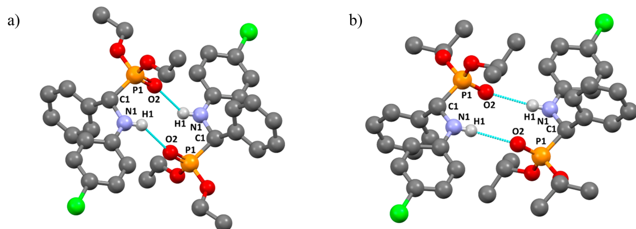
Figure 5. Molecular structures of 1 (a) and 11 (b) showing the labeling schemes of aminophosphonate groups and the hydrogen bonded rings formed by pairs of molecules in the crystals. H_{CH} hydrogen atoms omitted for clarity.
