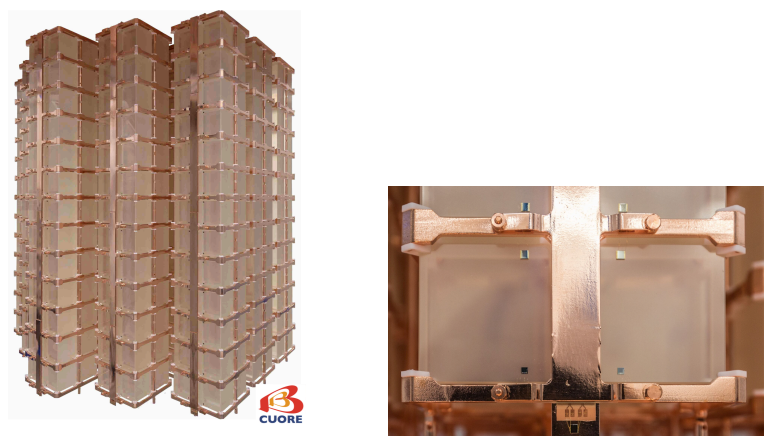
Fig. 1 [Left] The complete CUORE detector: the 19 towers hosting the 988 TeO 2 crystals. [Right] CUORE instrumented detectors: TeO 2 crystals held in the copper structure, Ge-NTD and Si-heater chips are glued on the crystals.
