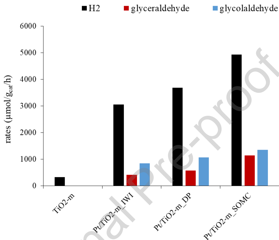
Figure 2. Rate of hydrogen production and liquid phase products for Pt NPs supported on TiO 2 -m by incipient wetness impregnation (IWI), deposition-precipitation (DP) methods and Surface Organometallic Chemistry approach (SOMC). 1M aqueous solution of glycerol, 30°C; 6 h, 0.5 g/L catalyst loading.
