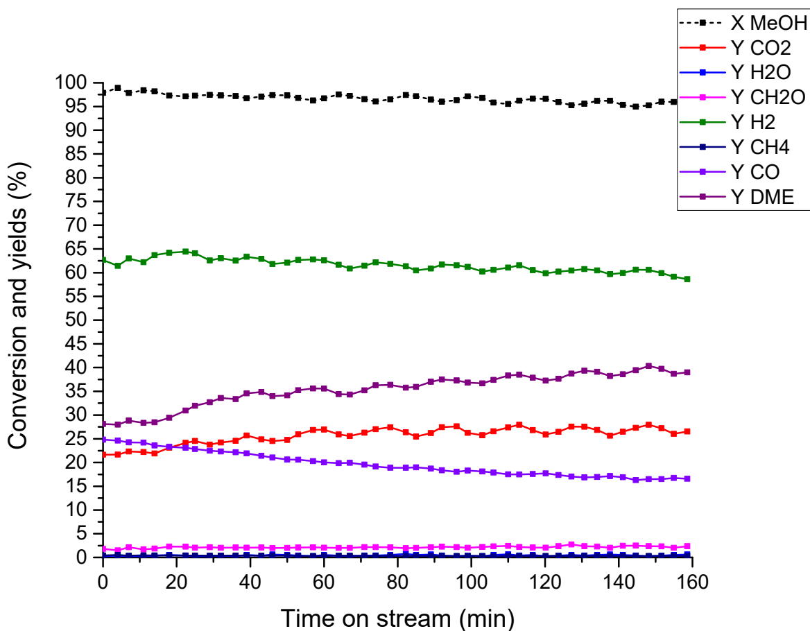
Figure 4: Methanol decomposition over \text{Ga}_2\text{O}_3 at 400^\circ\text{C} , \tau=1\text{s} , feed composition ( \text{CH}_3\text{OH}:\text{N}_2=18:82 )
