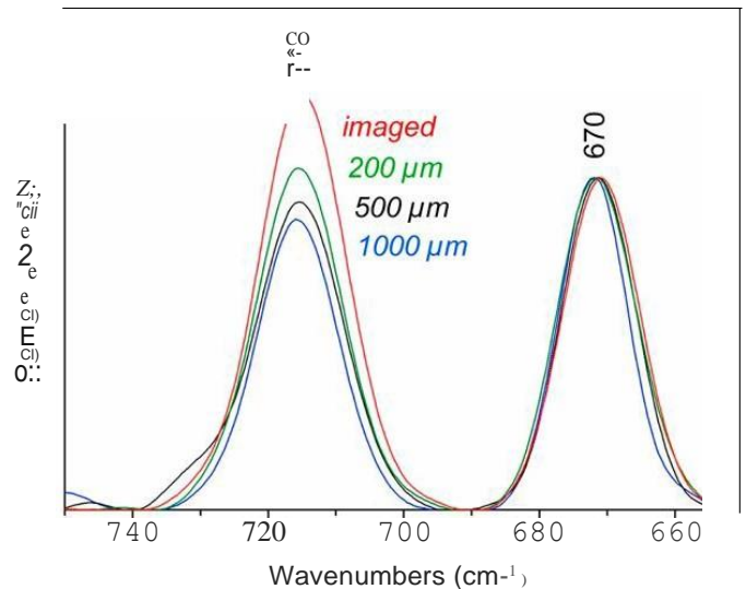
Fig. 6. Representative defocusing sequence of spectra acquired at t_0 on S3 and normalized to gypsum band at 670 \text{ cm}^{-1} . The micro-SORS steps are indicated (values typed in different colours). A progressive relative decrease of DES Raman band intensity is observed by increasing the defocusing distance. (For interpretation of the references to colour in this figure legend, the reader is referred to the Web version of this article.)
