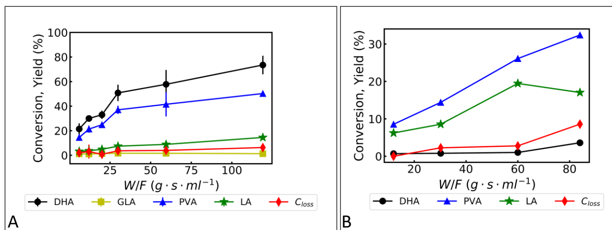
Figure 7. Product distribution over ZrPO as a function of W/F ratio feeding dihydroxyacetone (A) and pyruvaldehyde (B). Reaction conditions: A: 130 °C, 212-90 \mu m particle size, 10 bar, [DHA] = 0.4 M. B: 130 °C, 212-90 \mu m particle size, 10 bar, [PVA] = 0.4 M.
