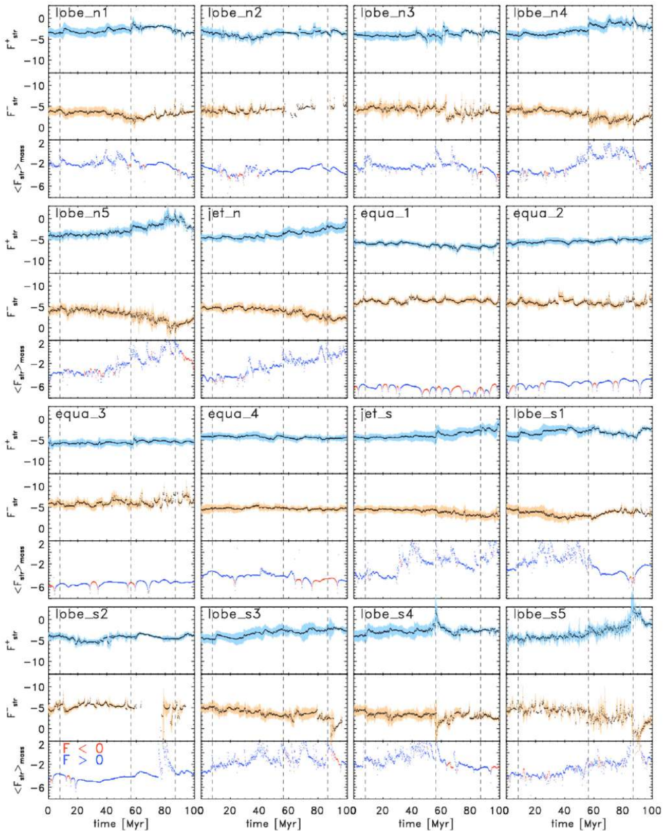
Figure 9. Lagrangian analysis: stretching term. Top and middle subpanels: evolution of the median \pm 1 standard deviation of the positive (blue) and negative (orange) component of the stretching term measured by the 16 different tracer families (see ID labels in the top-left corner). Bottom subpanel: mass-weighted mean stretching term measured by the tracers; a blue dot means the term is positive, while a red dot indicates a negative term. The unit of the y-axis is \log_{10}(\text{Myr}^{-3}) . The three vertical dashed lines mark the events of strongest entropy and correlated AGN power (Fig. 1).
