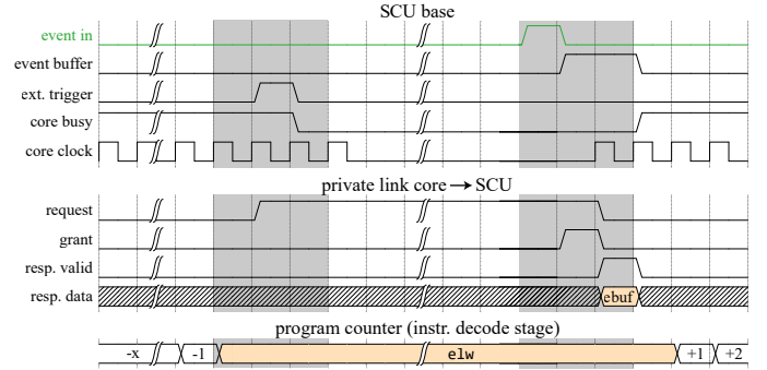
Fig. 4. Interfacing of the SCU with a RISC-V core and corresponding timing. Shaded intervals correspond to transitions to (left) and from (right) sleep state, respectively. The core executes a single instruction during the whole process. Note the absence of the grant (controlled by the SCU) until one cycle after an incoming event.
