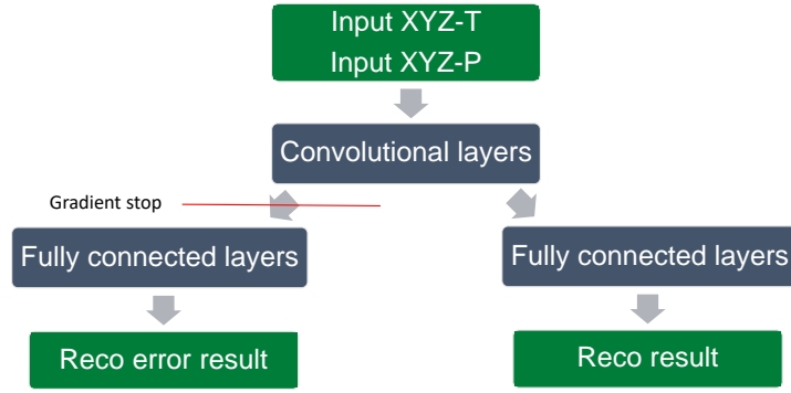
Figure 13. Scheme of the CNN architecture used for the event regressor. The properties of the convolutional layers and of the fully-connected network for the reconstruction of \vec{z}_{\text{reco}} is depicted in table 5 and in table 6.
