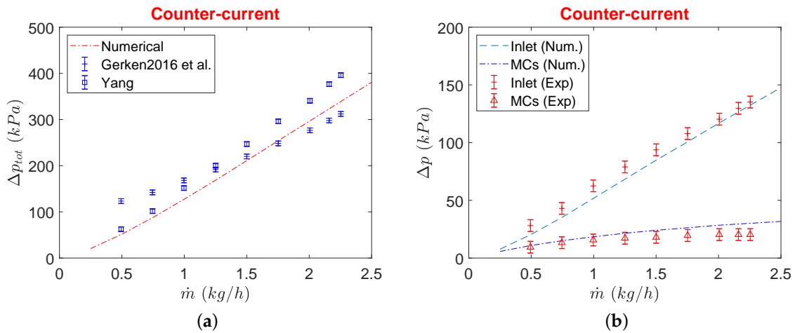
Figure 8. Comparison between experimental and numerical total pressure drop of \mu Hx (a), and in the inlet and MCs only (b).
