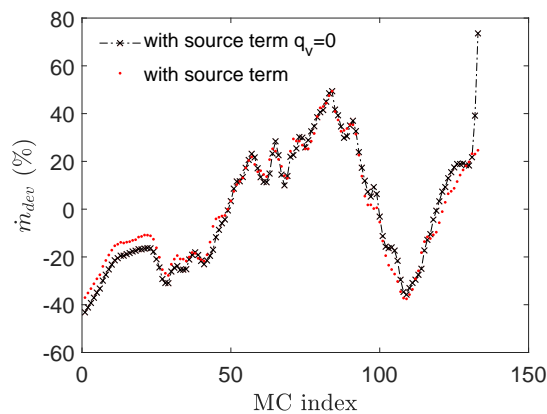
Figure 10. Flow maldistribution with (a) and without (b) source term q_v for counterflow configuration with \dot{m}_f = 2.5 kg/s.
