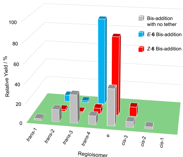
Figure 5. Relative reaction yields of the regioisomeric Bingel-Hirsch bis-adducts of E-6 (blue bars) and Z-6 (red bars) azobenzene tethers, in comparison with published data [8] in the absence of tethers (grey bars).
