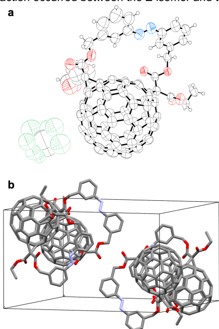
Figure 3. (a) Crystal structure (atomic displacement parameters are drawn at the 50% probability level) and (b) crystal packing (molecules of \text{CHCl}_3 are omitted for clarity) of the equatorial bis-adduct 1 .
