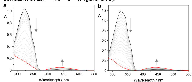
Figure 2. Absorption changes of azobenzene tethers E - 4 (a, 47 × 10 -6 M) and E - 6 (b, 44 × 10 -6 M) upon irradiation at 365 nm in toluene at room temperature.
