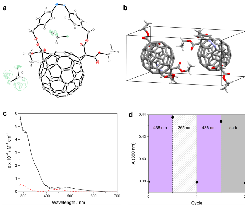
Figure 4. (a) Crystal structure (atomic displacement parameters are drawn at the 50% probability level) and (b) crystal packing (molecules of \text{CHCl}_3 are omitted for clarity) of equatorial bis-adduct 2 . (c) Absorption spectrum of 2 (black full line) in toluene, together with the spectra of Z-6 (red dashed line) and 7 (black dashed line). (d) Absorbance changes upon successive irradiations at 436 nm (purple areas) and 365 nm (striped area), and final rest in the dark (grey area).
