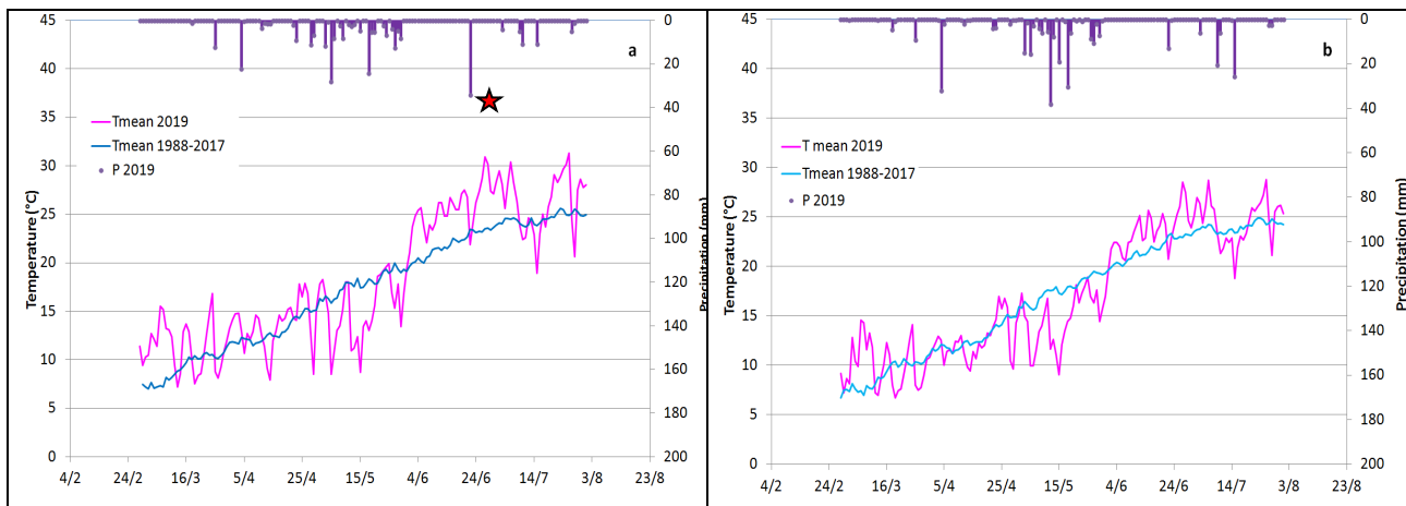
Figure 2: Meteorological data for the two experimental areas: a) DISTAL AG (BO); b) San Pietro in Vincoli VM (FC). As a reference, a line representing the 30 years mean air Temperature is added. The star shows the hailstorm that caused some damage to the plot (22 th of June)
