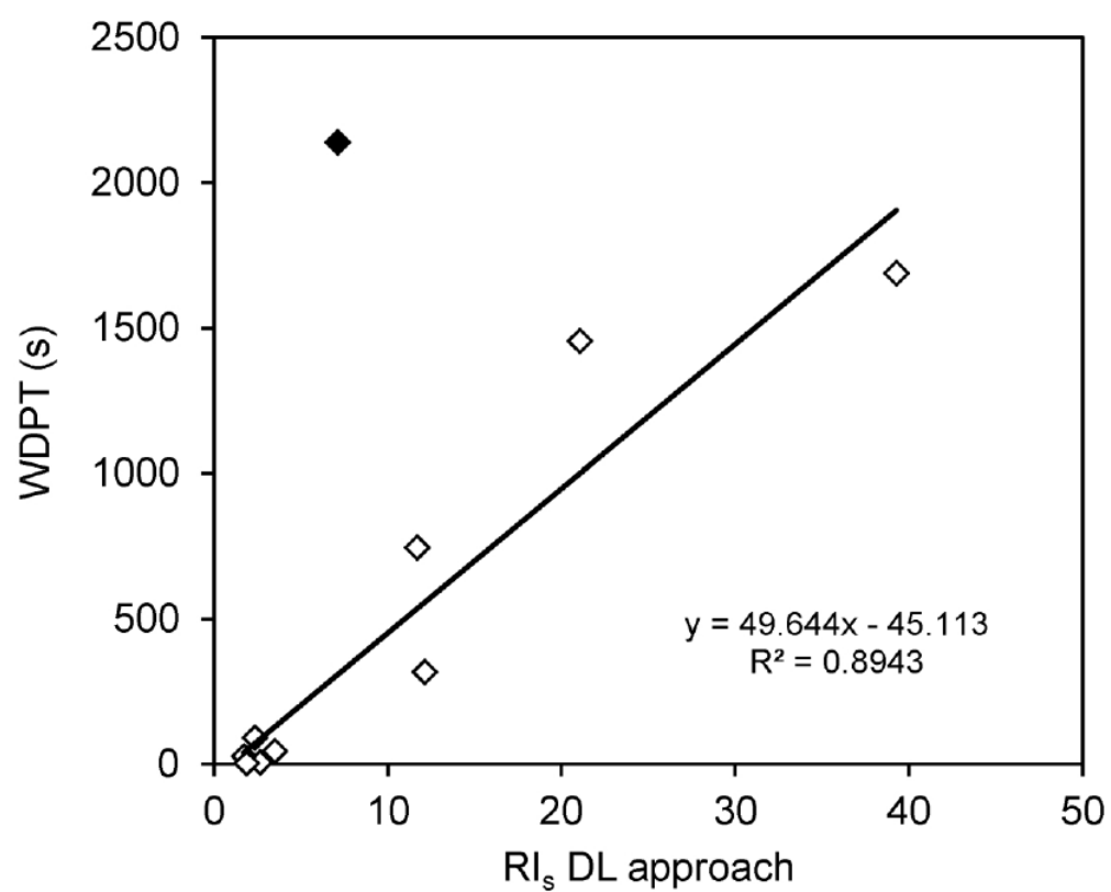
Figure 6 – Relationship between the repellency index RI_s calculated by the DL approach and the Water Drop Penetration Time (WDPT) for the different experimental conditions considered ( N = 9 ). Filled dot refers to the data collected in the organic layer of Javea forest site (H-O-D) that was excluded from the regression analysis
