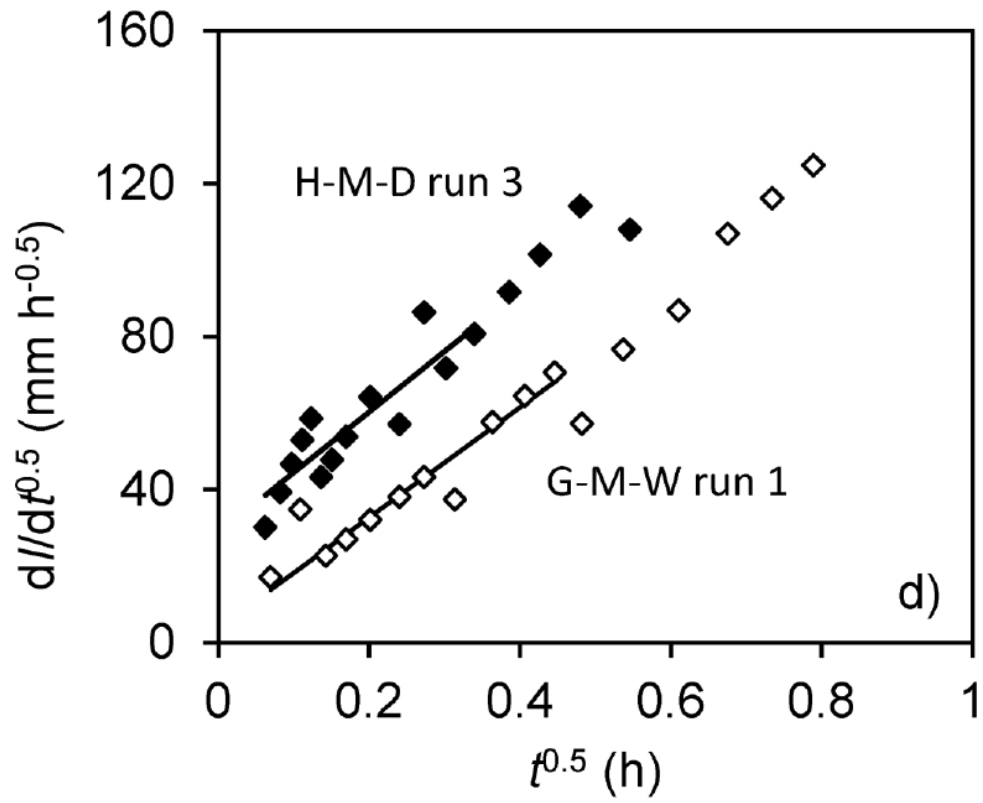
Figure 5 – Examples of application of cumulative linearization CL approach (a and b) and differentiated linearization DL approach (c and d) to water infiltration experiments in hydrophobic (a and c) and non-hydrophobic (b and d) soils
