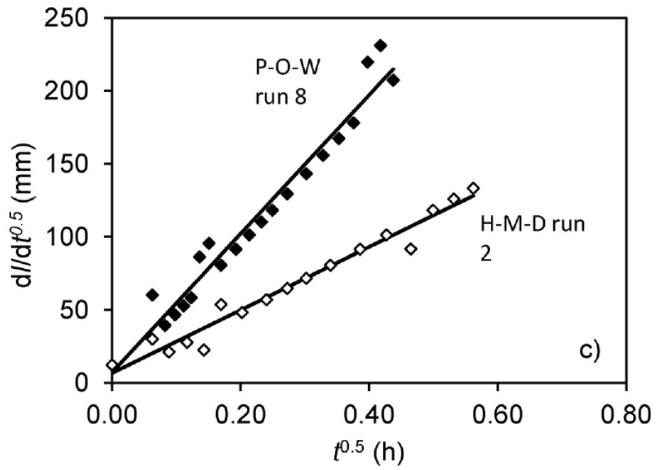
Figure 7 – Examples of cumulative ethanol infiltration curves plotted according to different representations: a) linearization of the early time infiltration data in the form I vs. t^{0.5} ; b) linearization of the complete infiltration curve according to CL approach; c) linearization of the complete infiltration curve according to DL approach
