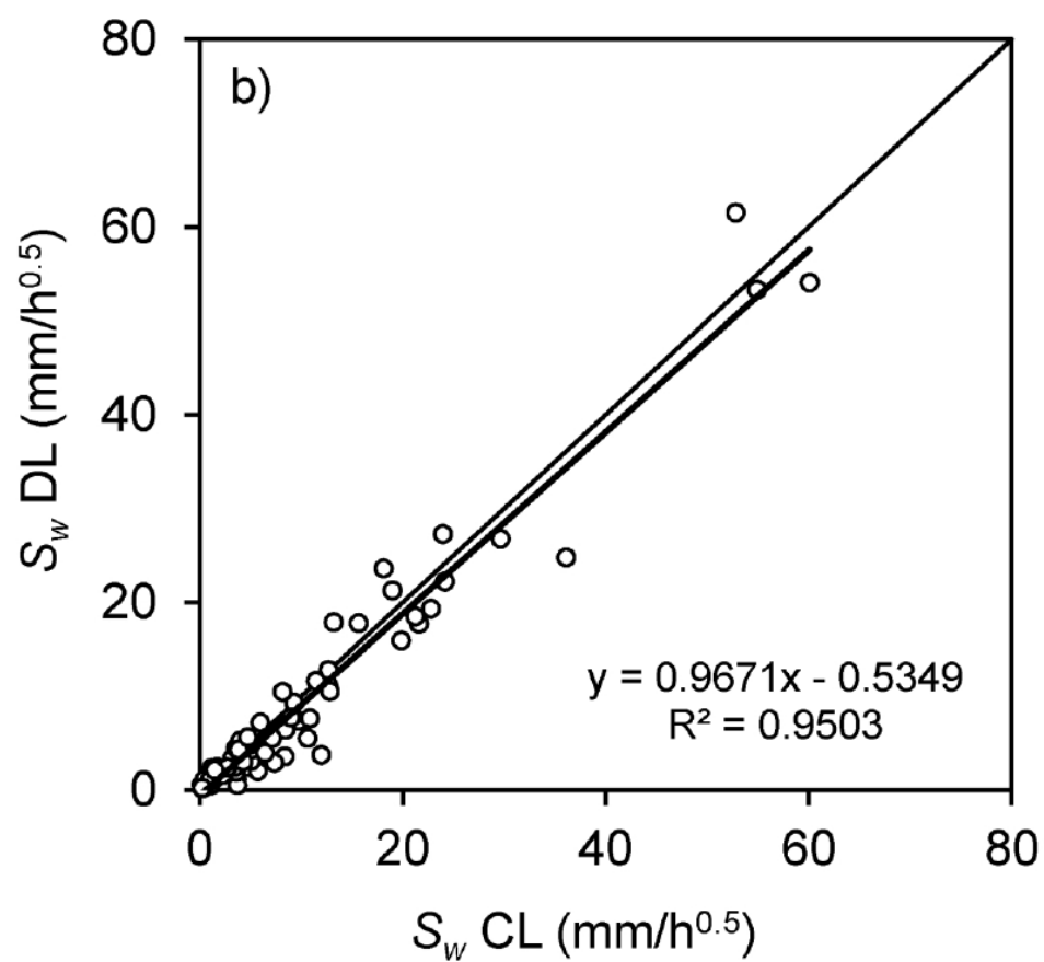
Figure 4 – Comparison between water sorptivity values, S_w , estimated according to different approaches: a) SL vs. CL, b) CL vs. DL
