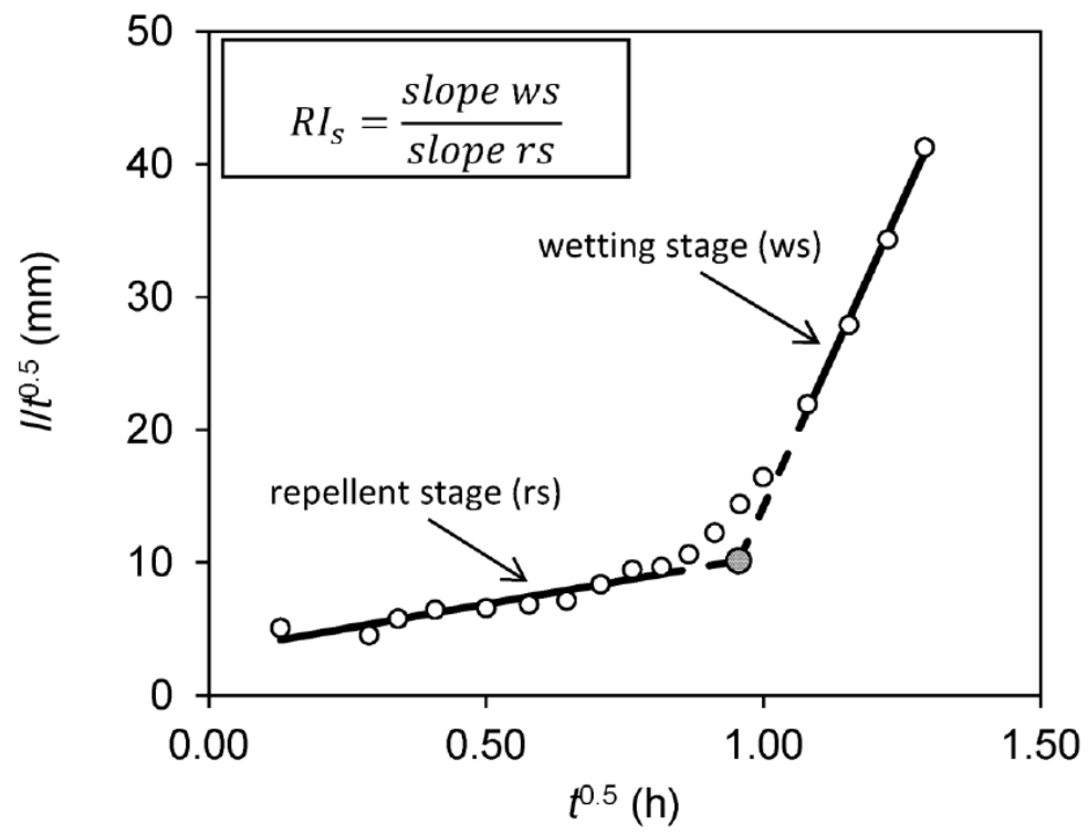
Figure 1 – Selection of the water repellent and wetting stages from linearized infiltration data (CL method).
