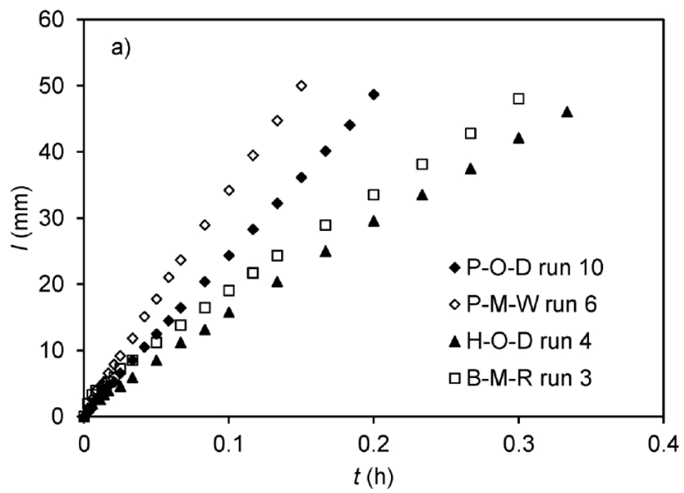
Figure 2 – Example of cumulative infiltration curves obtained in selected sites using a) ethanol and b) water as infiltrating fluid
