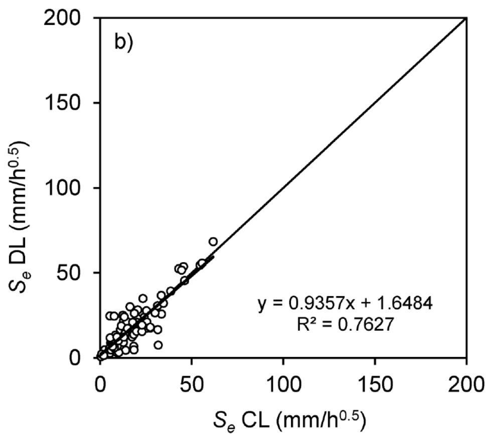
Figure 3 – Comparison between ethanol sorptivity values, S_e , estimated according to different approaches: a) SL vs. S1, b) CL vs. DL
