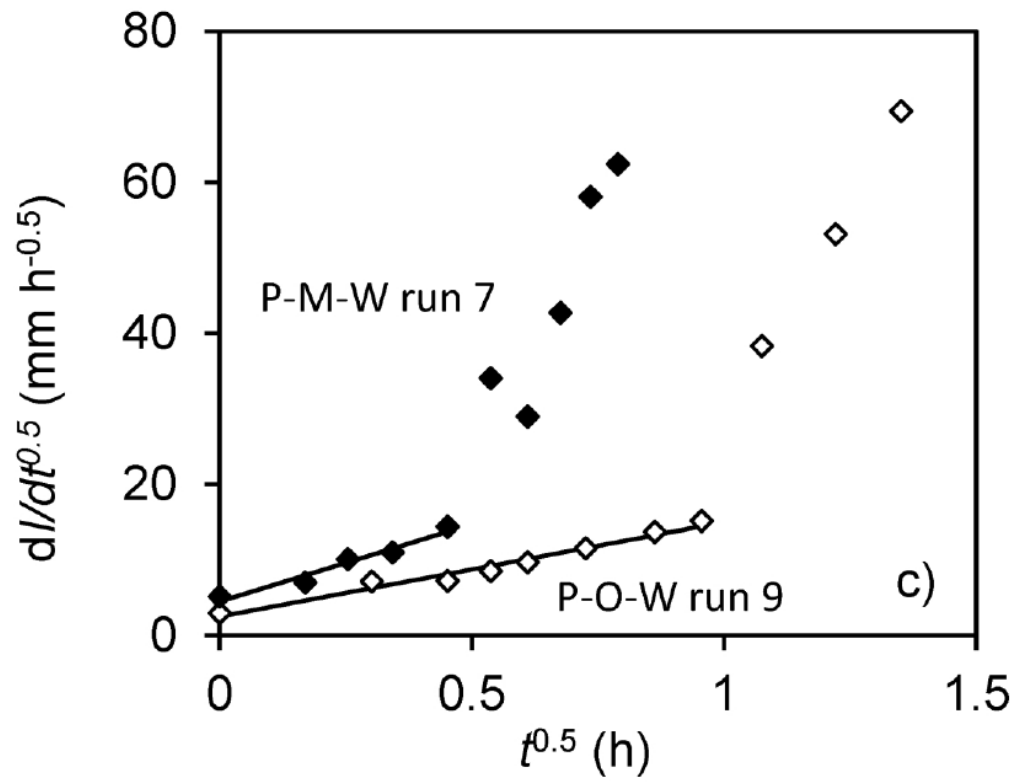
Figure 5 – Examples of application of cumulative linearization CL approach (a and b) and differentiated linearization DL approach (c and d) to water infiltration experiments in hydrophobic (a and c) and non-hydrophobic (b and d) soils
