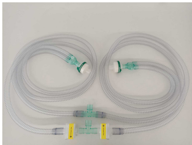
Figure 1 Assembled circuit.
