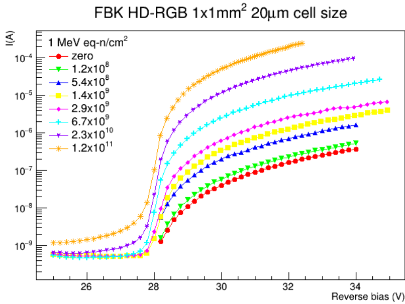
Figure 7: I-V curve of the 20 \mu m cell-pitch SiPMs. The value shown in the plot is normalized to one SiPM, i.e. the current from the PCB is divided by the number of SiPMs hosted in the board (9 SiPMs per board).
