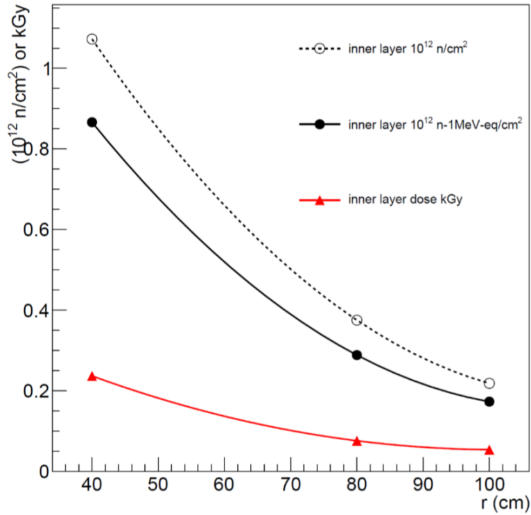
Figure 1: Ionizing doses (in kGy) and non-ionizing fluences (black dashed line: n/cm^2 ; black continuous line: 1 MeV-equivalent n/cm^2 ) as a function of the distance between the axis of the ENUBET decay tunnel and the inner radius of the calorimeter.
