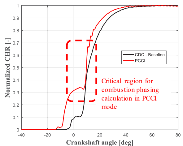
Figure 8: Normalized CHR curve for an engine cycle run at 2000 rpm and IMEP = 4 bar in PCCI mode.
