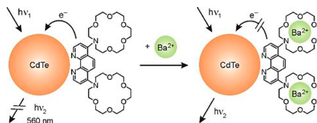
Figure 8. CdTe QDs functionalized with phenanthroline-azacrown ether ligands and scheme for the luminescent sensing of Ba^{2+} ions. [52]
