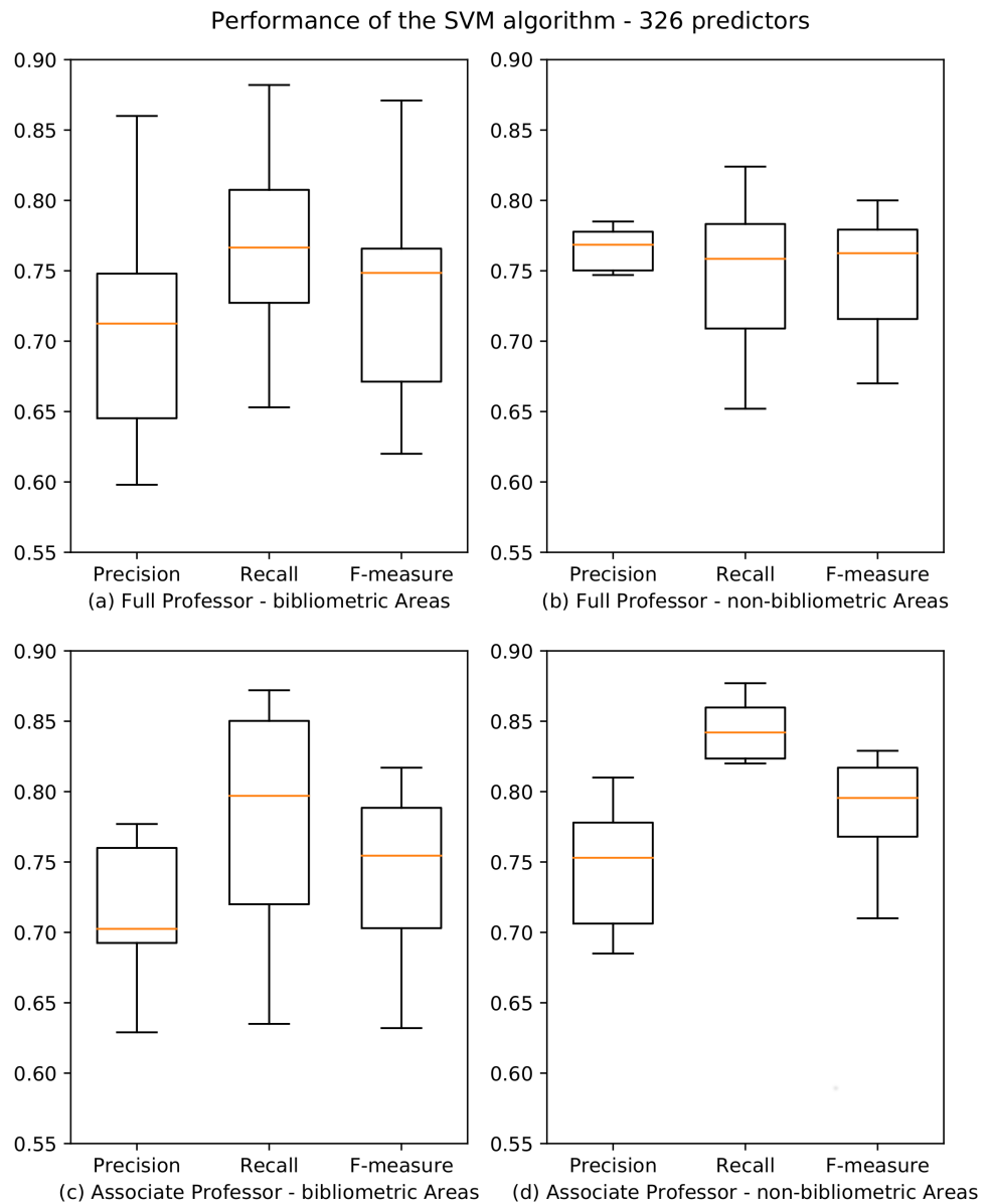
Figure 3 Boxplots depicting the performance of the SVM algorithm for academic level I and II. Precision, Recall and F-measure values are reported for bibliometric (A, C) and non-bibliometric (B, D) SAs. Full-size DOI: 10.7717/peerjcs.199/fig-3
