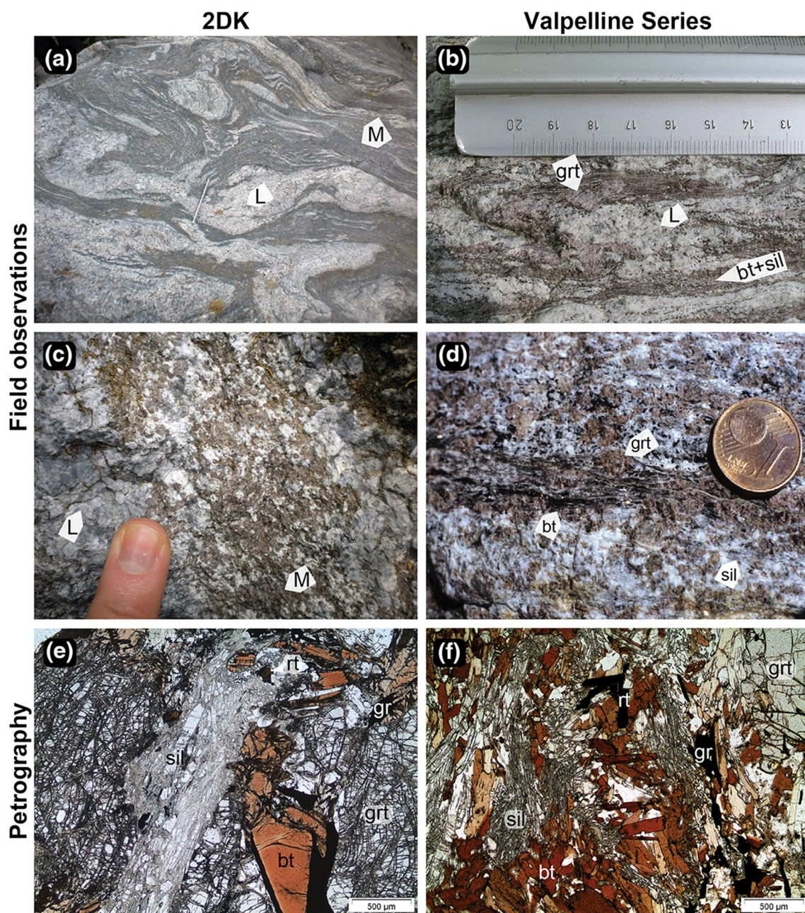
Fig. 2 Selected field and thin section photographs representative for the high-grade metasediments from the 2DK and Valpelline Series. a Migmatite typical of the central 2DK, with distinct leucosome (L) and melanosome (M) domains. b Migmatite from the Valpelline Series; L domains interlayered with garnet, biotite, and sillimanite schlieren. c L-rich migmatite with garnet, sillimanite, and biotite in M from the 2DK. d Garnet-rich migmatite from the Valpelline Series
