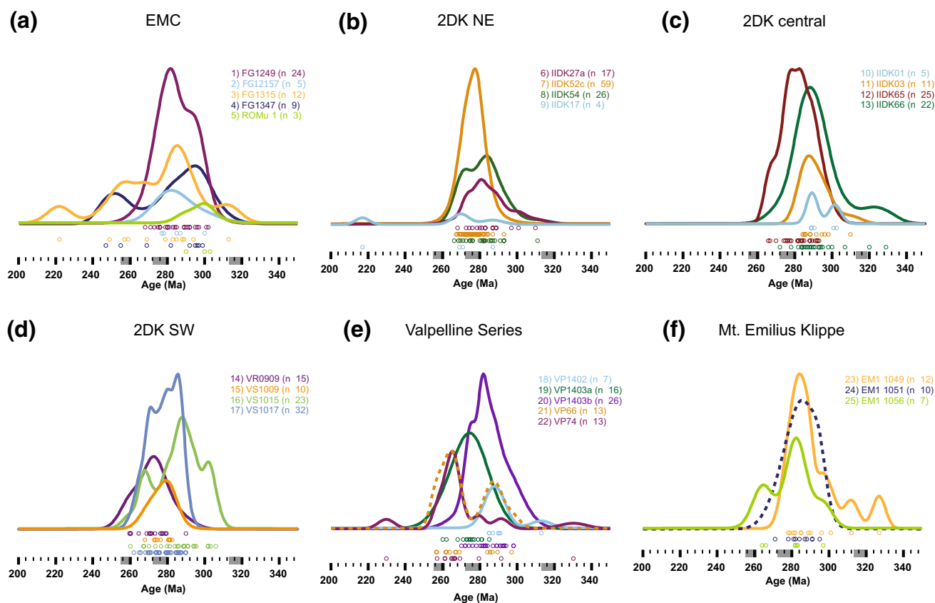
Fig. 4 Probability density plots for U/Pb zircon dates for individual samples from: a EMC, b 2DK NE, c 2DK central, d 2DK SW, e Valpeline Series, and f Mt. Emilius Klippe. Individual rock samples are
