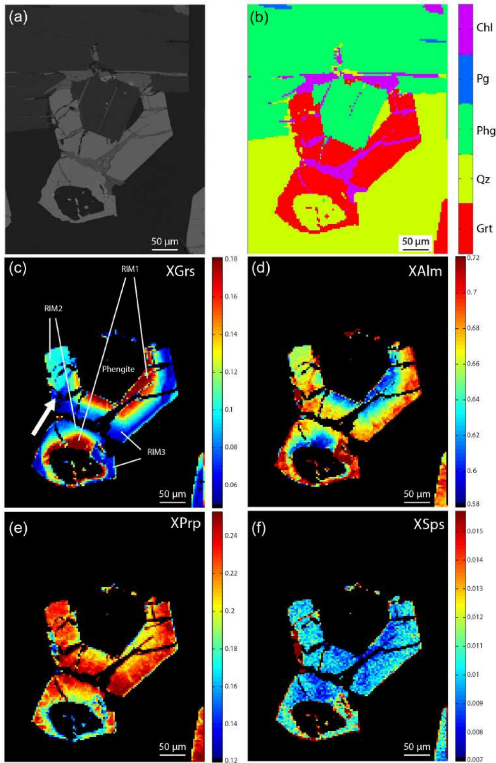
Figure 5. Small atoll garnet ( \varnothing \sim 100 \mu\text{m} ) in sample FG1315. (a) BSE picture. (b) Mineral phases (determined from X-ray maps). Note inclusions of quartz and phengite in the atoll core; fractures dissecting the entire garnet are filled by chlorite. Garnet occurs at the contact of quartz- and phengite-rich bands that define the main foliation. (c) Standardized X-ray map for the X_{\text{GrS}} endmember. Note the analogous zoning pattern as for large garnet (Fig. S5), with the same X_{\text{GrS}} contents and a Rim3 peninsula extending into the resorbed rims (arrow). (d–f) Standardized X-ray maps for X_{\text{Alm}} , X_{\text{Prp}} , and X_{\text{Sps}} , respectively.
