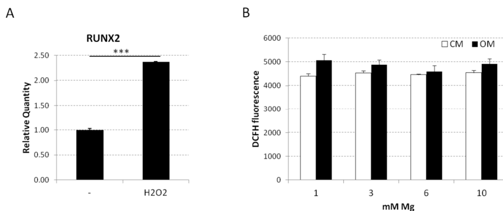
Figure 7. (A) The bMSCs were treated for 30 min with H_2O_2 (50 \mu M ) and then cultured for four days in culture medium (CM). RUNX2 expression was analyzed using QRT-PCR. The p -value was calculated vs. untreated cells; *** p < 0.001 . (B) Reactive oxygen species (ROS) accumulation was quantified using 2'-7'-dichlorofluorescein diacetate (DCFH, Sigma-Aldrich). Cells were seeded into black-bottomed 96-well plates (Greiner Bio-One) and cultured in 1, 3, 6, and 10 mM Mg, added or not with the osteogenic cocktail for 24 h. Then, cells were washed with phosphate-buffered saline (PBS) and exposed to DCFH (20 \mu M ). The rate of intracellular oxidative stress was evaluated by monitoring the emission at 529 nm of the DCFH dye using a GloMax ® -Multi Detection System (Promega, Madison, WI, USA). Three independent experiments were performed. Data are shown as means \pm standard deviation.
