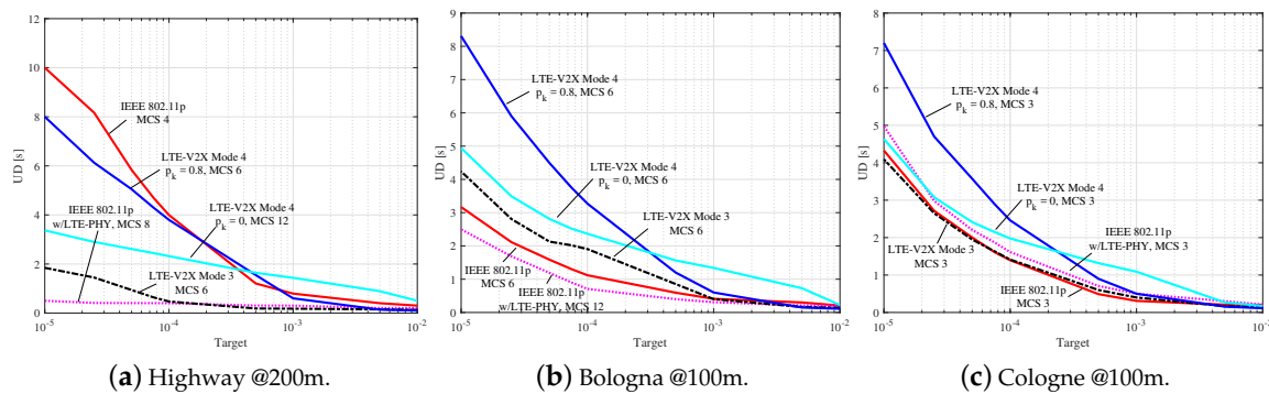
Figure 7. Update delay vs. target.
