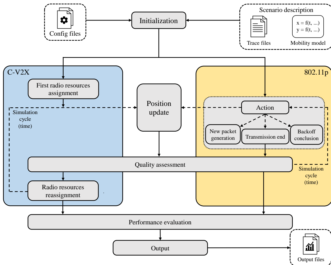
Figure 1. LTEV2Vsim block diagram.
