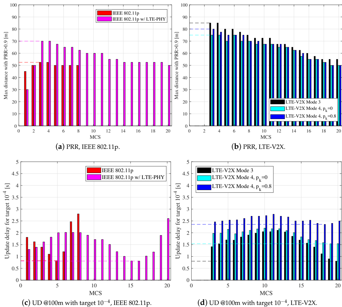
Figure 5. Packet reception ratio and update delay in Cologne.
