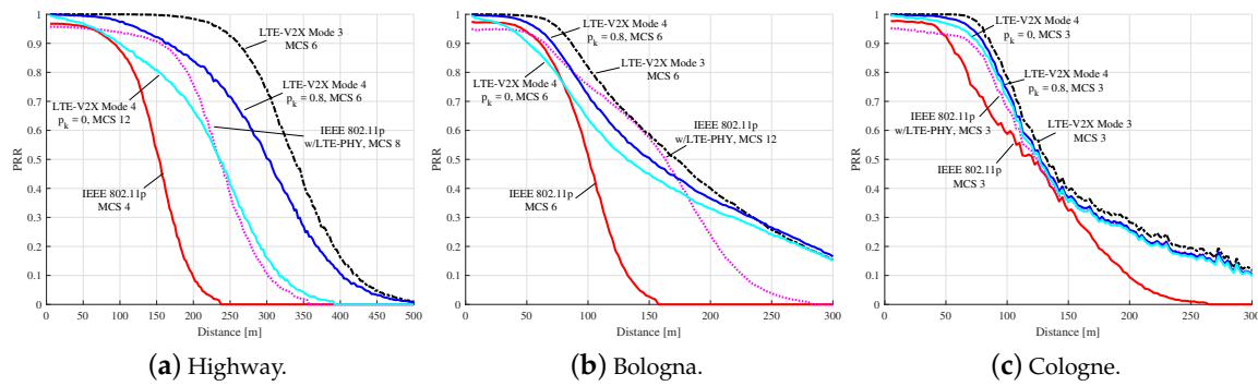
Figure 6. Packet reception ratio vs. distance.
