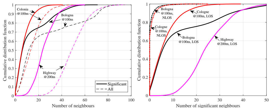
(a) Significant vs. all neighbours. (b) Significant neighbours in LOS vs. NLOS.
