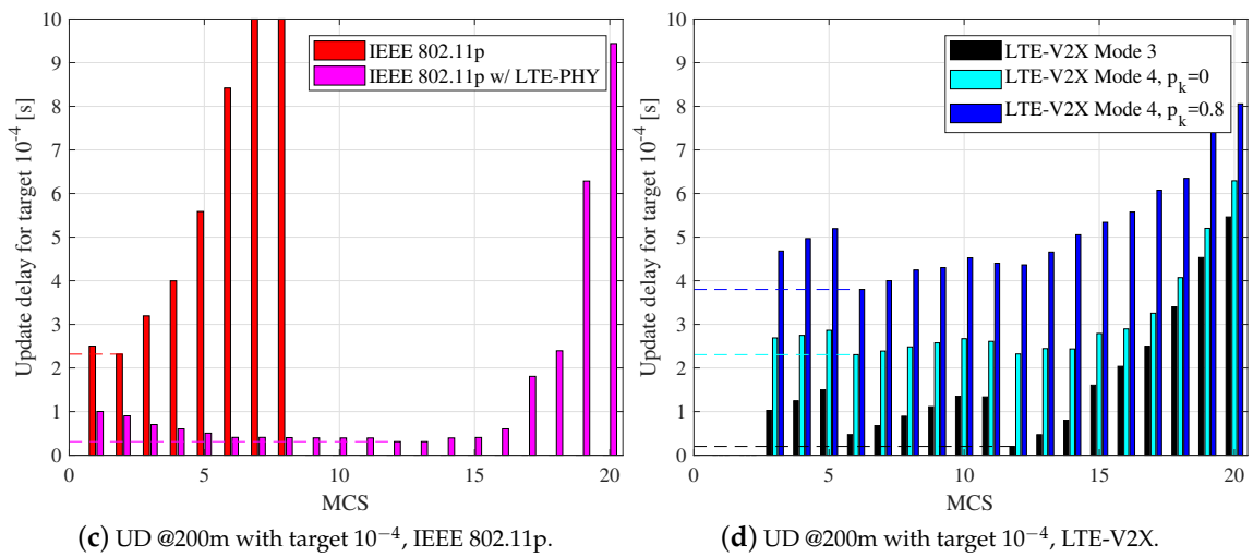
Figure 3. Packet reception ratio and update delay in Highway.
