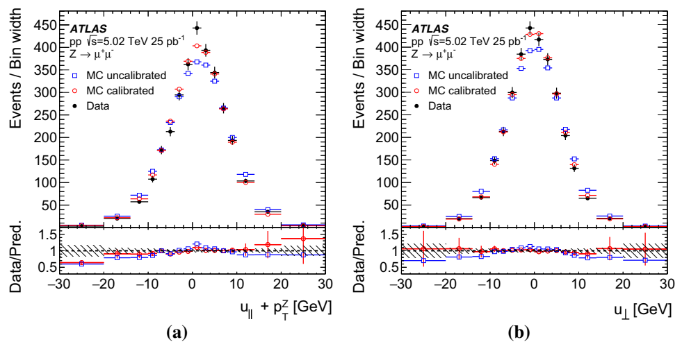
Fig. 3 Distributions of a u_{\parallel} + p_T^Z and b u_{\perp} in data and Z \rightarrow \mu^+ \mu^- MC simulation before (squares) and after (circles) recoil calibration. The shaded band in the ratio panels represents the statistical uncertainty of the data sample, while the error bars represent the systematic uncertainty associated with the calibration procedure
