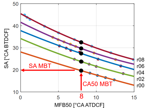
Figure 10. SA Maximum Brake Torque (MBT) determination procedure.
