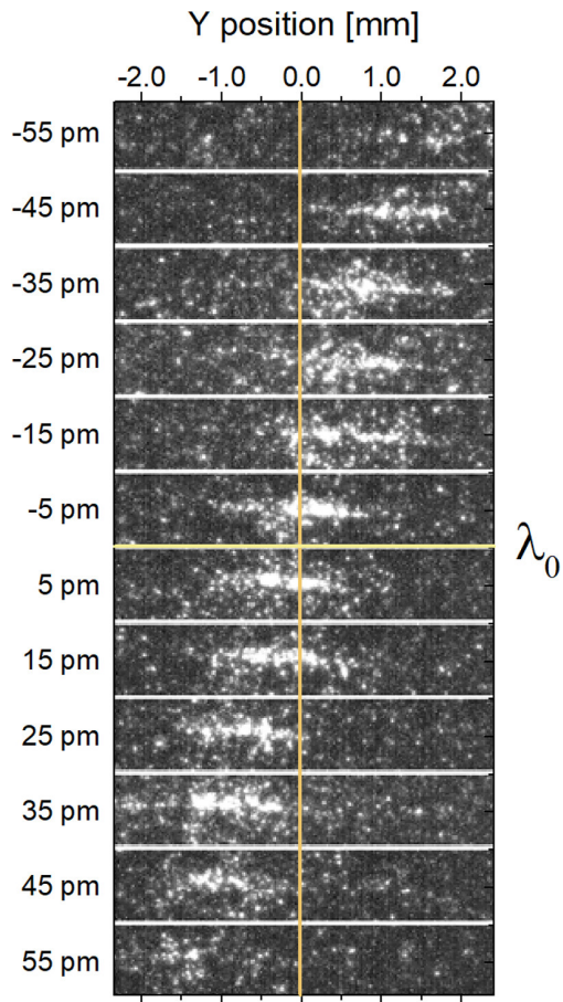
FIG. 5. images of spatial distribution in the plane transverse to the 1.0 T field (x- y plane, see Fig. 2) of e^+ freed by Ps photoionization. Each image corresponds to different wavelengths of the UV laser pulse. The detune of the wavelength with respect to \lambda_0 is reported on the left side.
