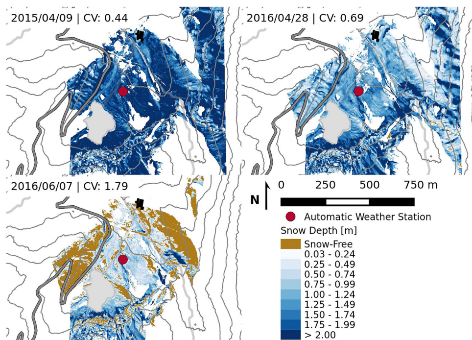
Figure 4. Temporal dynamics and within-site variations of SD. TLS maps for peak accumulation in 2015 and 2016 and the melting season 2016.
