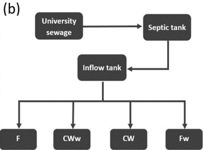
Fig. 1 Pilot plant in March 2016 (a) and a schematic representation of the water flow in the system (b). F Filter, CWw constructed wetland with earthworms, CW constructed wetland, Fw Filter with earthworms. All the systems are vertical flow
