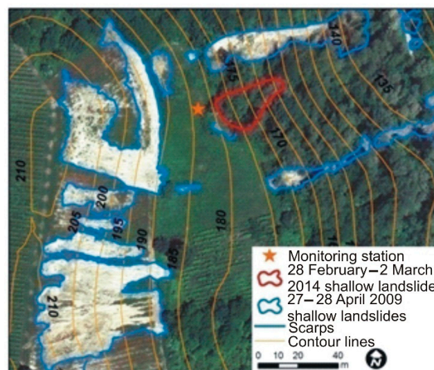
Figure 2. Detailed view of the testsite slope where the monitoring station was installed, showing evidence of the shallow landslides triggered during the 27–28 April 2009 event. The aerial photograph of the area was captured by Ditta Rossi s.r.l. (Brescia, Italy) on 18 May 2009.
