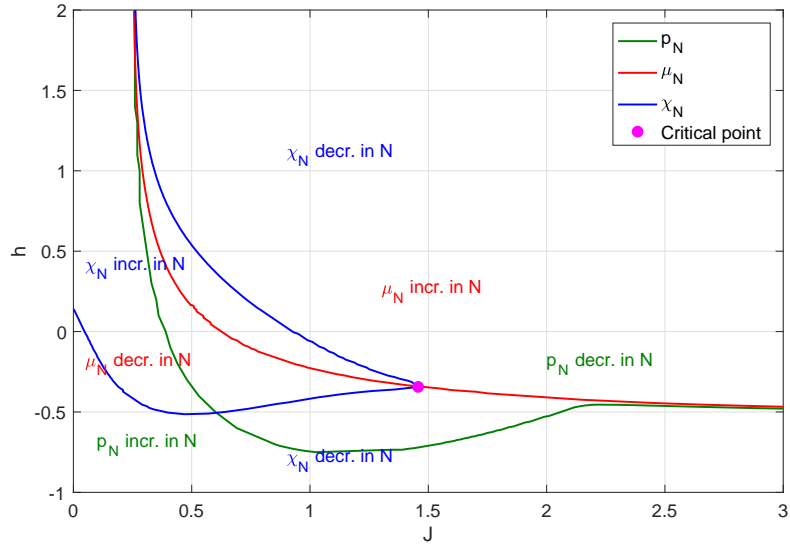
Figure 1: Phase space (J, h) . The green curve represents the values (J, h) for which the pressure density p_N changes monotonicity with respect to N (i.e. \Lambda changes sign). The red curve represents the values (J, h) for which the average monomer density \mu_N changes monotonicity with respect to N (i.e. \Lambda' changes sign). The blue curve represents the values (J, h) for which the susceptibility \chi_N changes monotonicity with respect to N (i.e. \Lambda'' changes sign). The purple dot is the critical point of the system.
