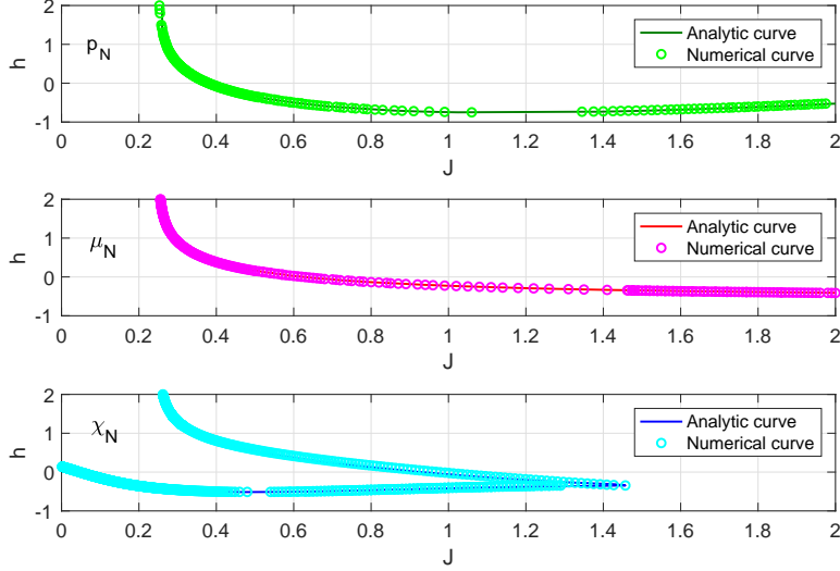
Figure 2: Phase space (J, h) : comparison between analytical and numerical monotonicity (with respect to N ) curves for the pressure density p_N (upper panel), for the average monomer density \mu_N (middle panel) and for the susceptibility \chi_N (lower panel). The analytical curves (continuous lines) are the same as in Fig. 1.
